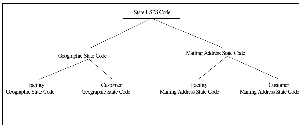
Figure 1 — Specialization/generalization hierarchy.
