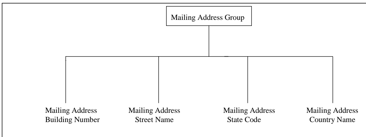
Figure 2 — Decomposition/aggregation example.
